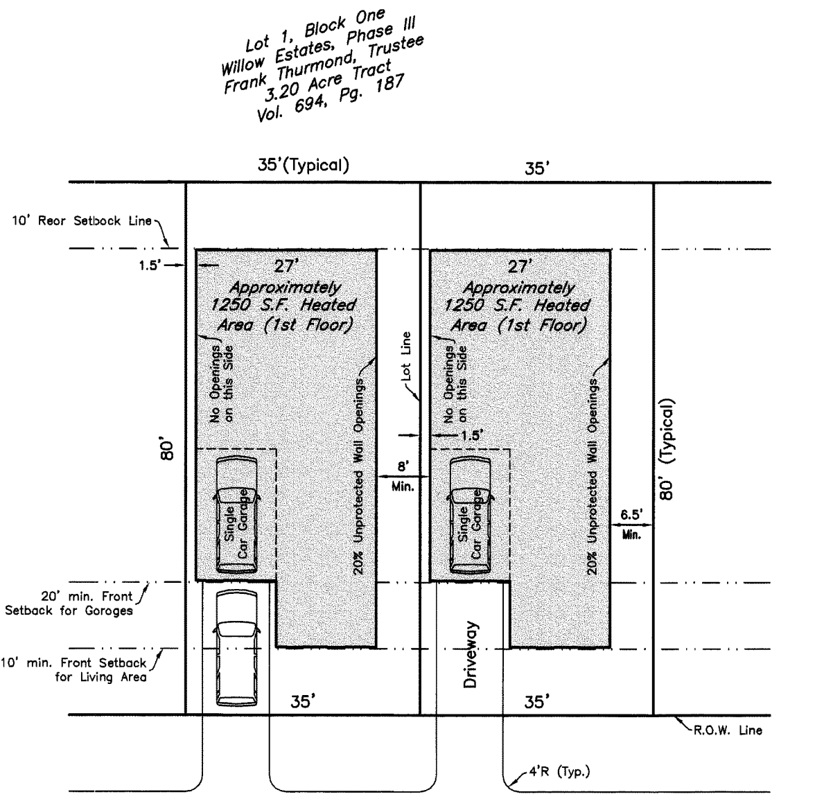
TYPICAL LOT PLAN ~ BLOCKS 3, 4 & 5 Scale: 1" = 20'
