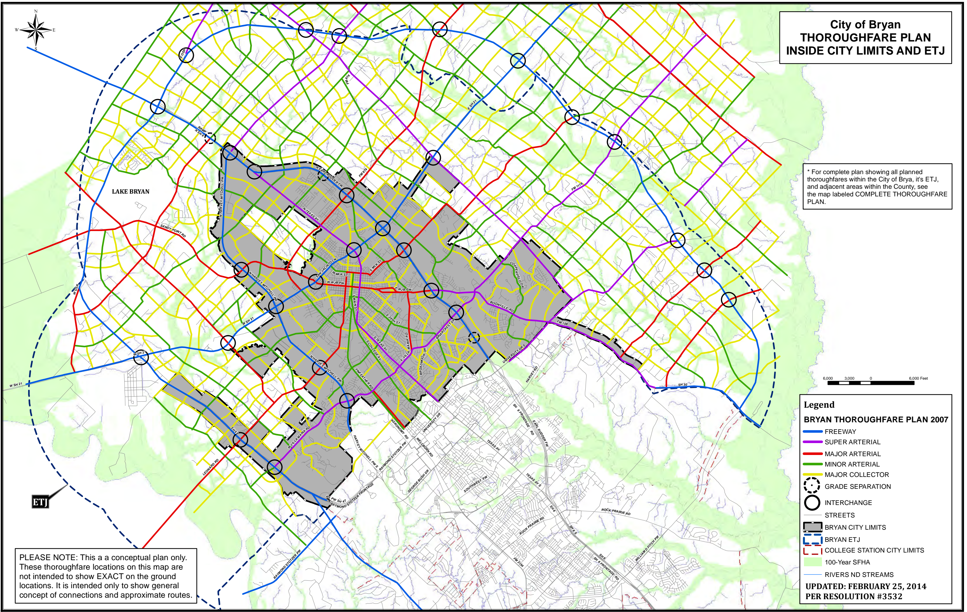
Figure 6-3 Thoroughfare Plan - Inside City Limits and ETJ
